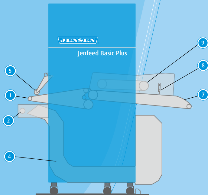
Side view Jenfeed Basic Plus with optional deep vacuum box and divided conveyor
