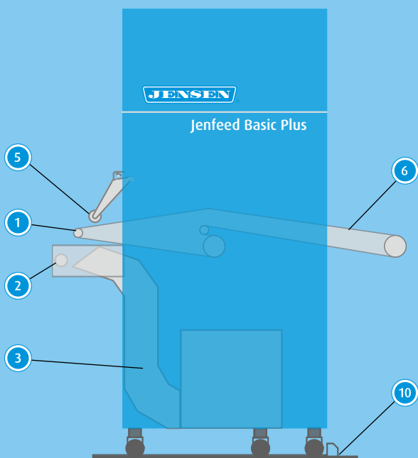
Side view Jenfeed Basic Plus with standard vacuum box and standard conveyor
